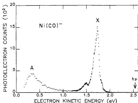
Figure 1. Photoelectron spectrum of \text{Ni}(\text{CO})^- obtained with 2.540-eV photons; ion current was about 18 pA. Peak X corresponds to the transition to ground-state \text{Ni}(\text{CO}) which defines the electron affinity.
