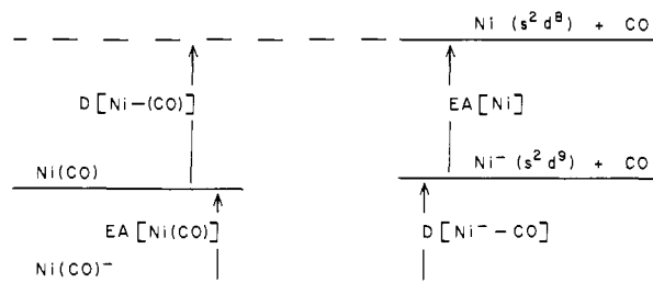
Figure 4. Illustration of the energetic relationship between the negative ion \text{Ni}(\text{CO})_n^- and neutral \text{Ni}(\text{CO})_n , from which eq 6 is derived.
