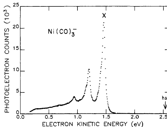
Figure 3. Photoelectron spectrum of \text{Ni}(\text{CO})_3^- obtained with 2.540 eV photons and an ion current of 6.0 nA; the electron affinity is again determined from the peak labeled X.
